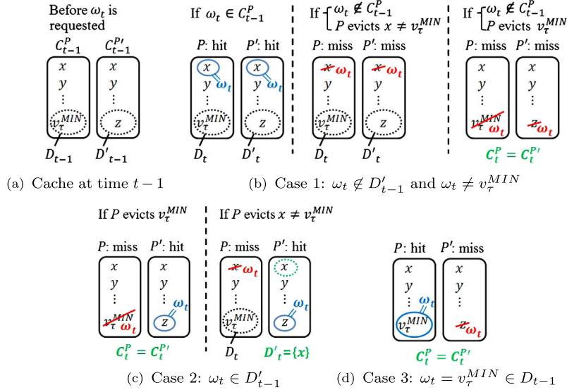
Fig. 1. Change of cache states at time t according to the request of \omega_t .
