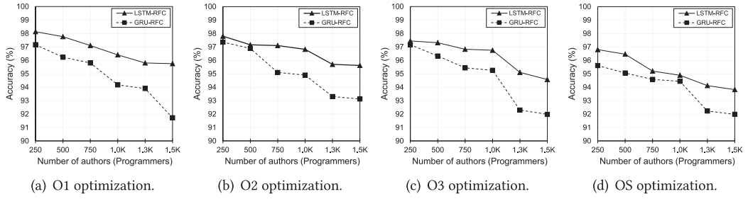
Fig. 10. The accuracy of the authorship identification of programmers using their binary samples compiled with different optimization options, showing promising accuracy results even with decompiled binary samples.
