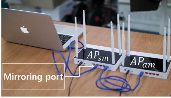
Fig. 9. PrAP's hardware. AP_{sm} is a WLAN router associated with a legitimate AP, and AP_{am} is a WLAN router disguised as a legitimate AP.
