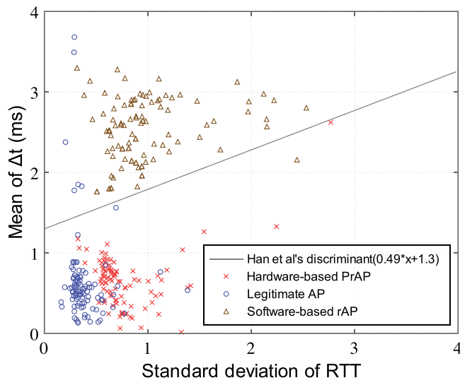
Fig. 14. Results of Han et al.'s [3] algorithm for two rogue APs, a software-based rAP and a hardware-based PrAP.
