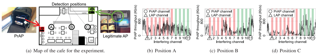
Fig. 24. Legitimate AP serving in channel 1. Rogue AP relayed the Internet service of the legitimate AP and served as a trusted AP (using a cafe's wireless network SSID) in channel 11. In position A, the PrAP-Hunter was close to the PrAP. In B, the PrAP-Hunter had the same distance with both the legitimate AP and the PrAP. In C, the PrAP-Hunter was close to the legitimate AP.
