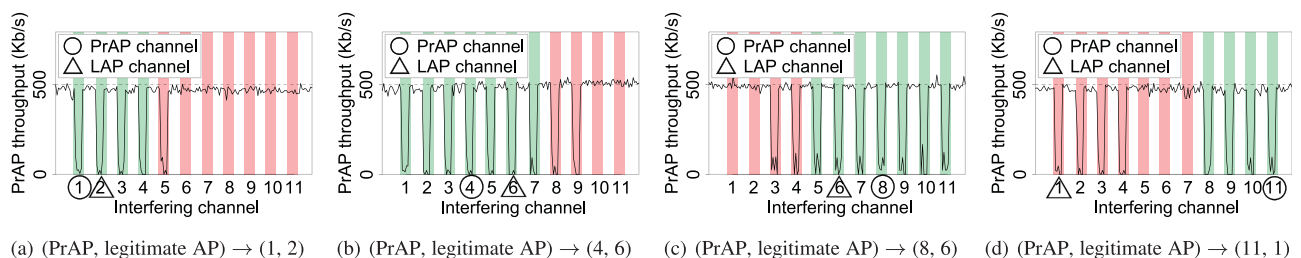
Fig. 6. Cases of a PrAP existence varying the channel of the PrAP and of the legitimate AP. Red bars indicate the non-overlapped channels. The non-overlapped channels are affected by interference with the channel of the connecting AP (here, a PrAP).
