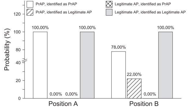
Fig. 19. A plot examining the accuracy (measured by the true positive, true negative, false positive and false negative) of our detection algorithm at different positions.
