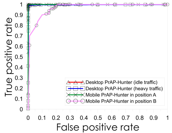
Fig. 22. The receiver operating characteristic (ROC).
