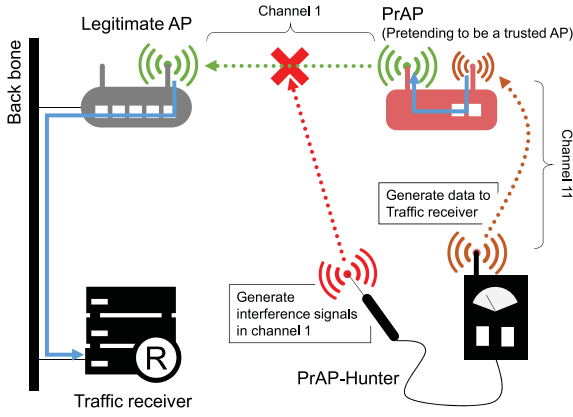
Fig. 3. A legitimate AP on channel 1 and a PrAP repeating signals of the legitimate AP on channel 11. The PrAP-Hunter generates traffic to the traffic receiver through the PrAP. The interference device interferes with channel 1. An AP is said to be rogue if we observe obstruction of traffic on channel 11 via the PrAP-Hunter.
