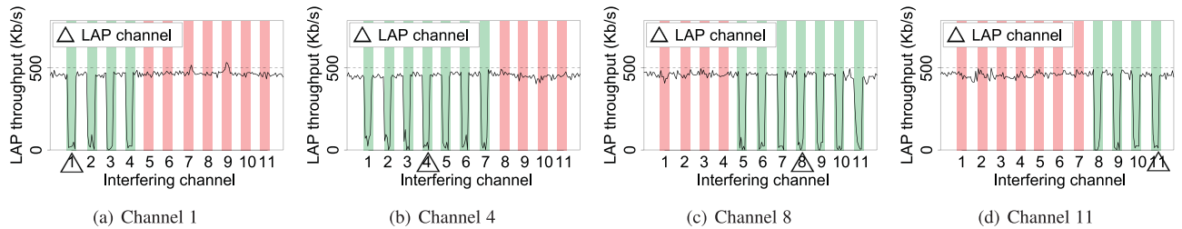
Fig. 5. Cases of only a legitimate AP on various channels. Green bars indicate the overlapped channels with the connecting AP's (here, a legitimate AP) channel affected by interference, which confirms the channel overlapping model of IEEE802.11n.
