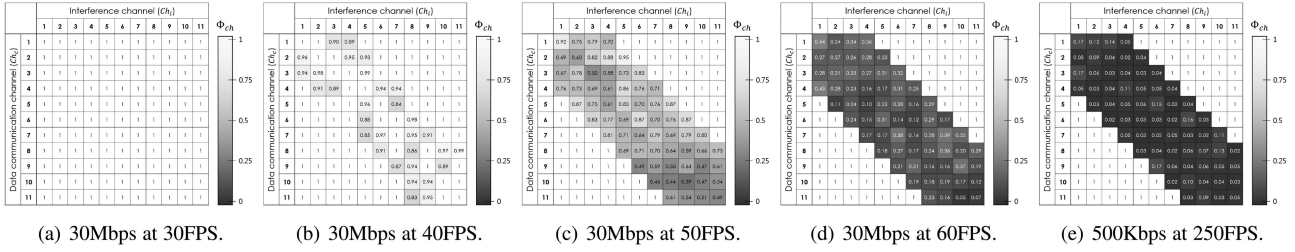
Fig. 7. Examining the performance of modified beacon frame's interference under different conditions. Shaded blocks are affected channels by interference. Darker blocks represent more interference.
