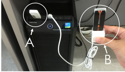
Fig. 10. Hardware setting of the desktop PrAP-Hunter. A is an wireless interface that is connected to the target AP and generates traffic, and B is the wireless interface that sends interference signals through 2.4 GHz channels.
