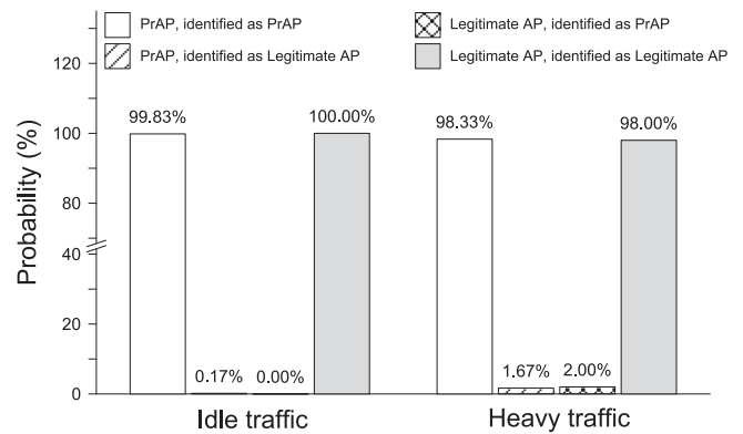
Fig. 15. Examining the accuracy of our detection algorithm in different traffic scenarios.
