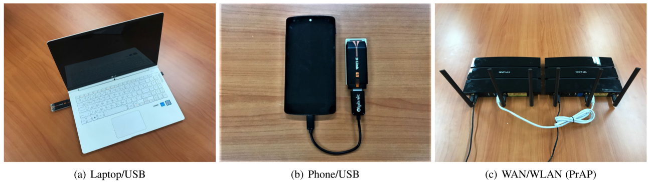
Fig. 2. Three ways of setting up a rogue AP (rAP), using a universal serial bus (USB)-based wireless interface (along with the built-in wireless interface) as in (a) with a laptop and (b) with a phone, and using a physical layer connector of two routers (PrAP) as in (c).
