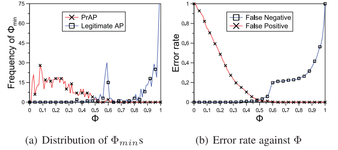
Fig. 18. (a) Desktop PrAP-Hunter: Distribution of \Phi_{min} s; heavy traffic. y -axis ( = f(\Phi_{min}) ) shows the frequency of \Phi_{min} . (b) CDF of false negative and false positive rates against \Phi .
