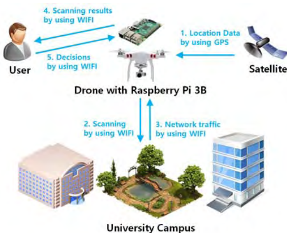
Fig 2 Flowchart for a study of flying intrusion detector using the drone
